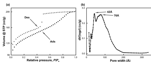
Figure 3. a) Nitrogen sorption isotherm of Se-3D , b) pore size distribution profile of Se-3D .
